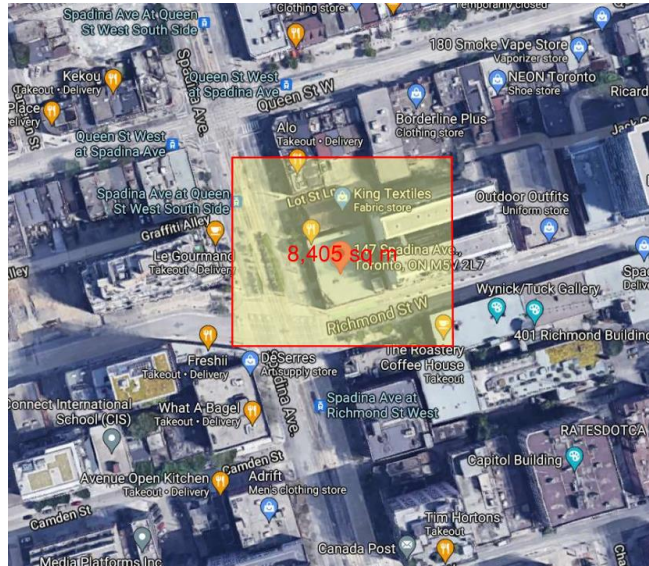
Figure 7 - Solar PV Area Required to Offset Highest Performance Energy
